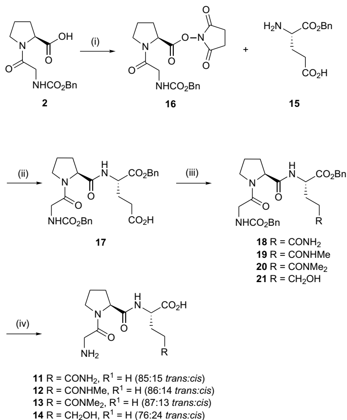
Scheme 4. Reagents and conditions: (i) DME, N -hydroxysuccinimide, DCC, N 2 , 0°C, 23 h (85%); (ii) Et 3 N, H 2 O, THF, rt, 16 h (95%); For 11 : (iii) Boc 2 O, NH 4 HCO 3 , pyridine, 1,4-dioxane, N 2 , rt, 21 h (89%); (iv) H 2 , 10% Pd/C, 2:1 MeOH–H 2 O, rt, 18 h (82%). For 12 : (iii) Et 3 N, MeNH 2 ·HCl, CH 3 CN, TBTU, N 2 , rt, 16.5 h (79%); (iv) H 2 , 10% Pd/C, 2:1 MeOH–H 2 O, rt, 18 h (67%). For 13 : (iii) Et 3 N, Me 2 N·HCl, CH 2 Cl 2 , EtOCOCl, N 2 , 0°C to rt, 17 h (89%); (iv) H 2 , 10% Pd/C, 2:1 MeOH–H 2 O, rt, 18 h (95%). For 14 : (iii) (a) Et 3 N, THF, EtOCOCl, N 2 , –5°C, 30 min; (b) NaBH 4 , MeOH, –5°C to rt, 30 min (63%); (iv) H 2 , 10% Pd/C, 82:16:2 THF–H 2 O–Et 3 N, rt, 18 h (100%).
