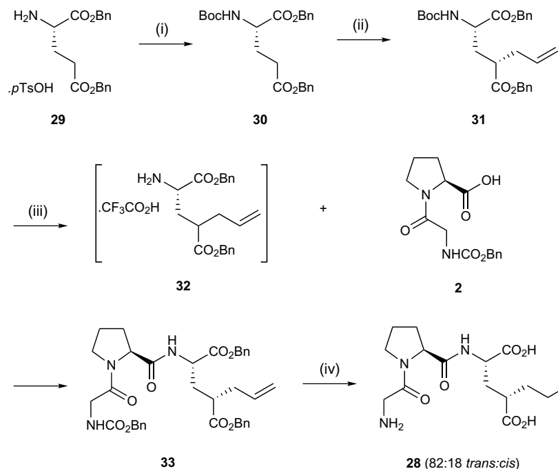
Scheme 7. Reagents and conditions: (i) \text{Et}_3\text{N} , \text{Boc}_2\text{O} , \text{CH}_2\text{Cl}_2 , 0^\circ\text{C} to rt, 19 h (97%); (ii) (a) lithium hexamethyldisilazide, THF, -78^\circ\text{C} , \text{N}_2 , 40 min; (b) allyl bromide, -78^\circ\text{C} , 1.5 h then -78^\circ\text{C} to rt, 1.5 h (73%); (iii) (a) TFA, \text{CH}_2\text{Cl}_2 , 0^\circ\text{C} , 2 h; (b) \text{CH}_2\text{Cl}_2 , \text{Et}_3\text{N} , \text{EtOCCl} , 0^\circ\text{C} to rt, \text{N}_2 , 17 h (87%); (iv) \text{H}_2 , 10% Pd/C, 2:1 MeOH– \text{H}_2\text{O} , 18 h (77%).
