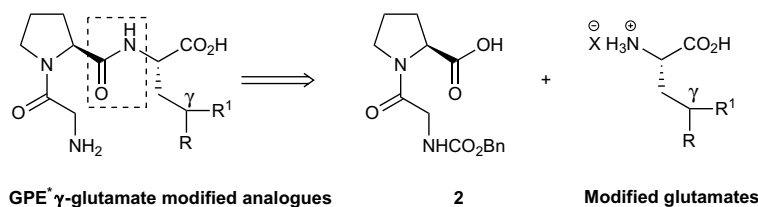
Scheme 1. General retrosynthesis for GPE* \gamma -glutamate modified analogues.
